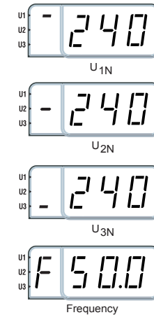
Figure 3: Display for L-N setting. 240V and 50.0Hz shown as example
